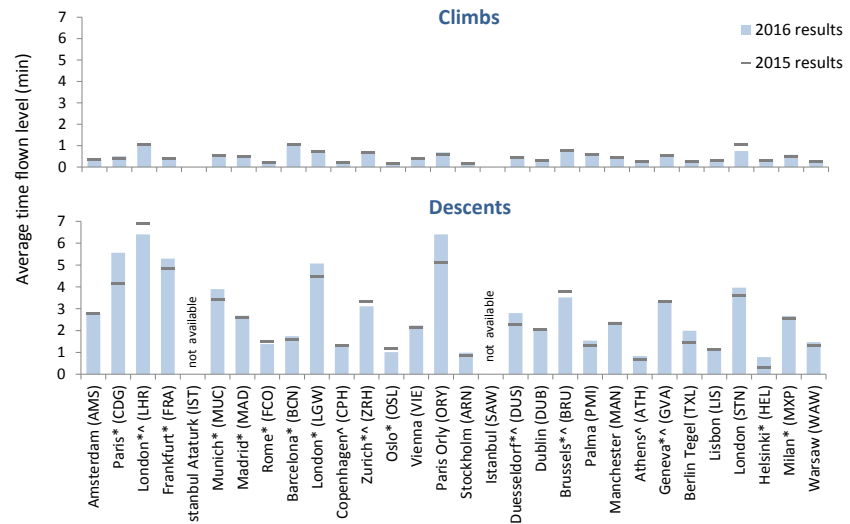
Figure 4-14: Average time flown level per flight at the top 30 airports
