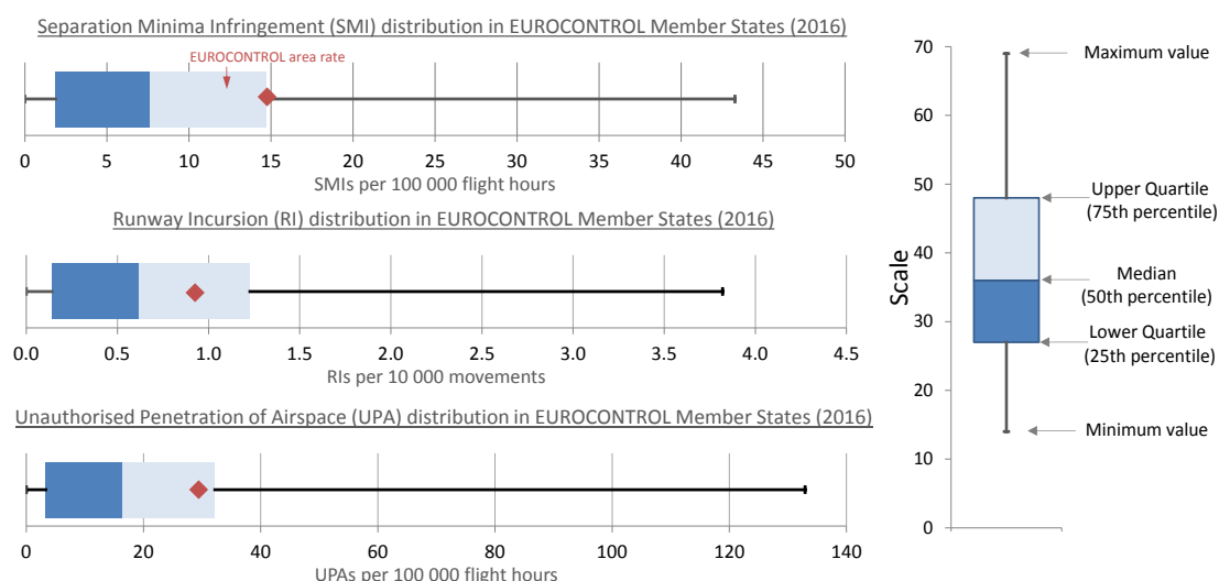
Figure 2-4: Occurrence rates EUROCONTROL area (2016P)
