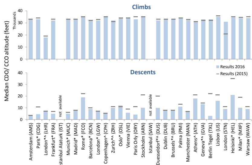
Figure 4-15: Median CDO/CCO altitude at the top 30 airports
