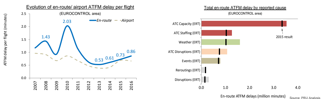
Figure 3-3: Average en-route ATFM delay (EUROCONTROL area)
